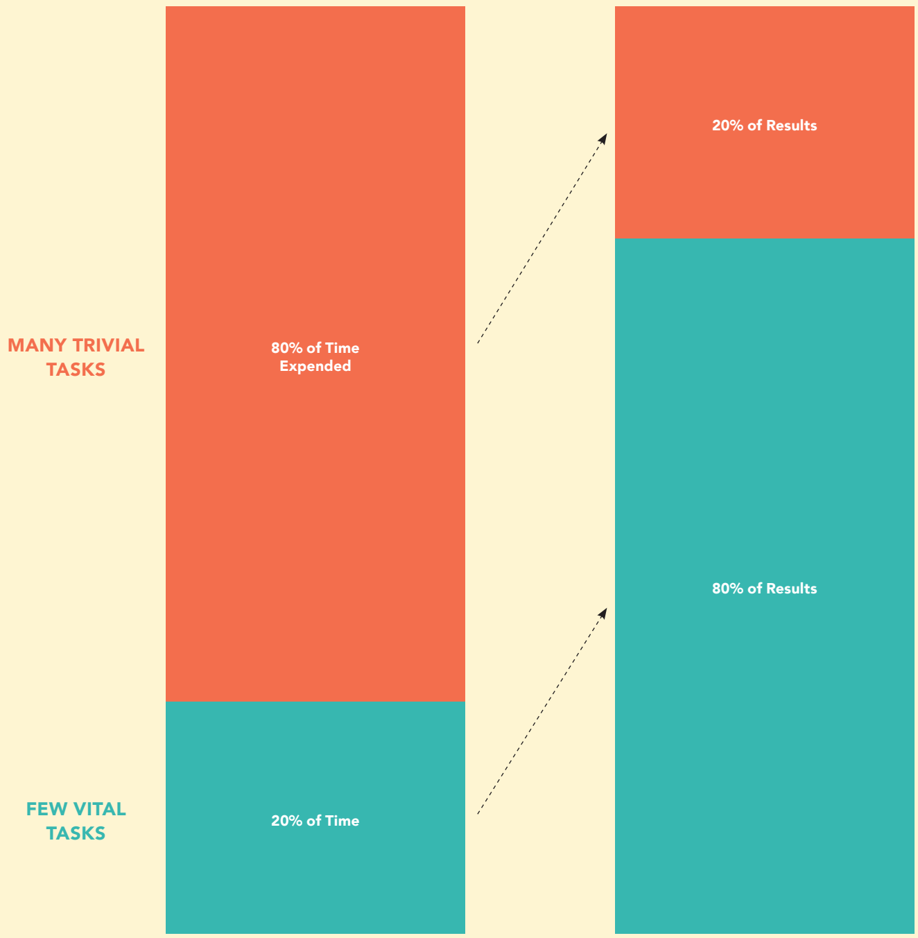
Figure 1 Pareto Principle
